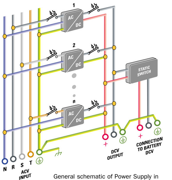
General schematic of Power Supply in parallel with external general static switch.
